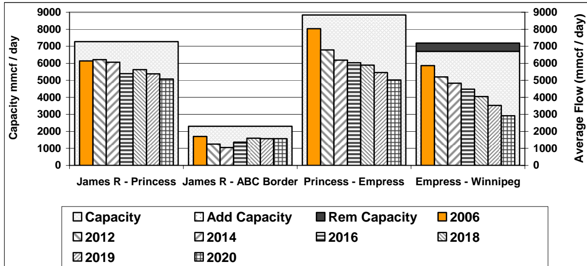
Figure 4.18 Scenario #3 (TCPL/Alliance Transportation) Section Volumes and Capacities (Alberta Southeast)
