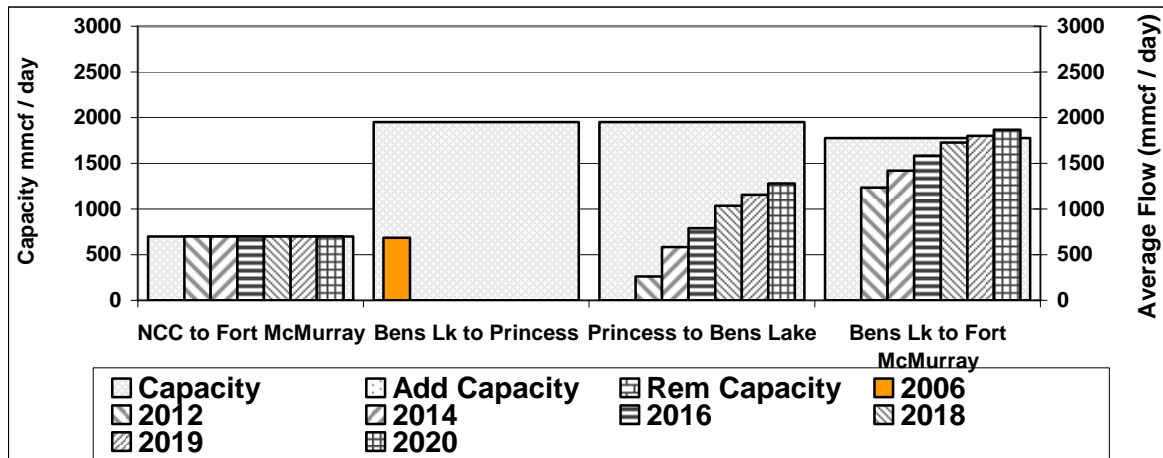
Figure 4.9 Scenario # 1 (Utilizing TCPL Integrated System) Section Volumes and Capacities (Fort McMurray)
