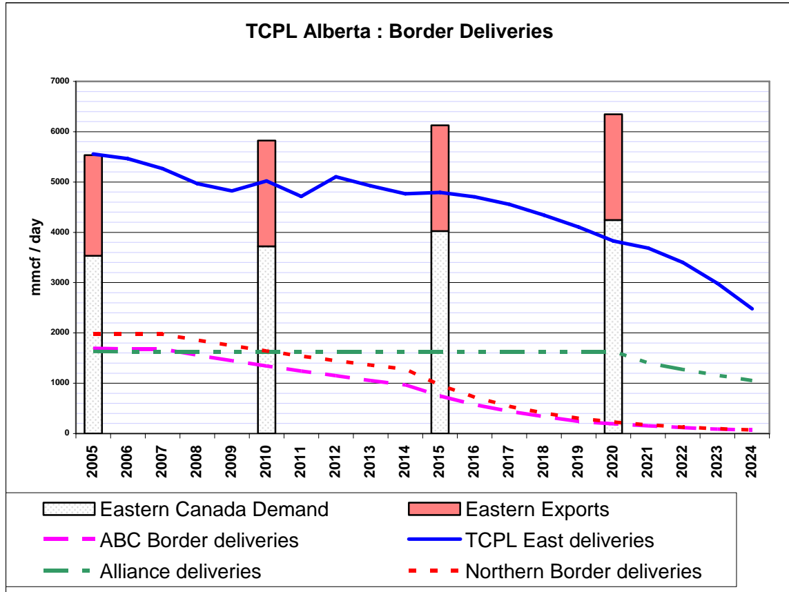
Figure 4.5 TCPL East Canadian Demand and Export Potential
