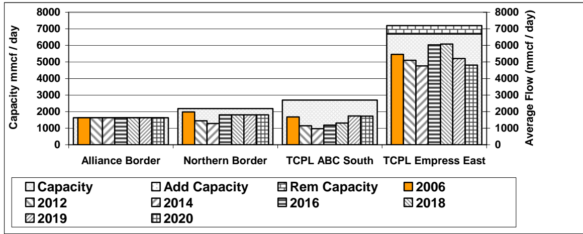
Figure 4.6 Scenario #1 (Utilizing TCPL Integrated System) Border Deliveries versus Export Capacity
