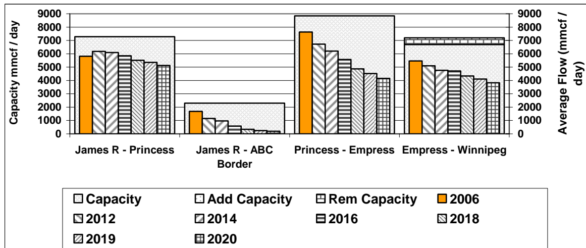
Figure 4.3 Base Case Section Volumes and Capacities (Alberta Southeast)
