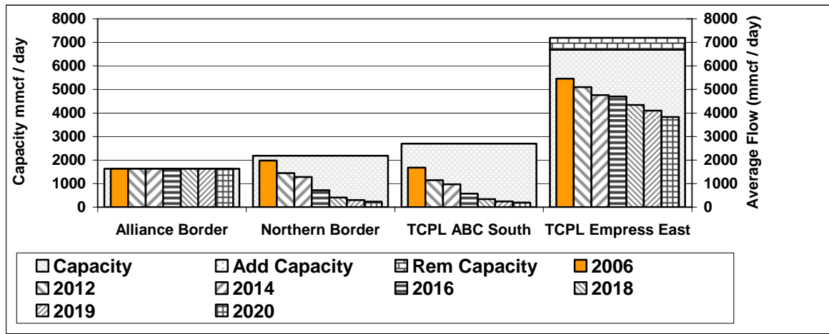
Figure 4.1 WCSB Export Pipeline Base Case Border Deliveries versus Export Capacity
