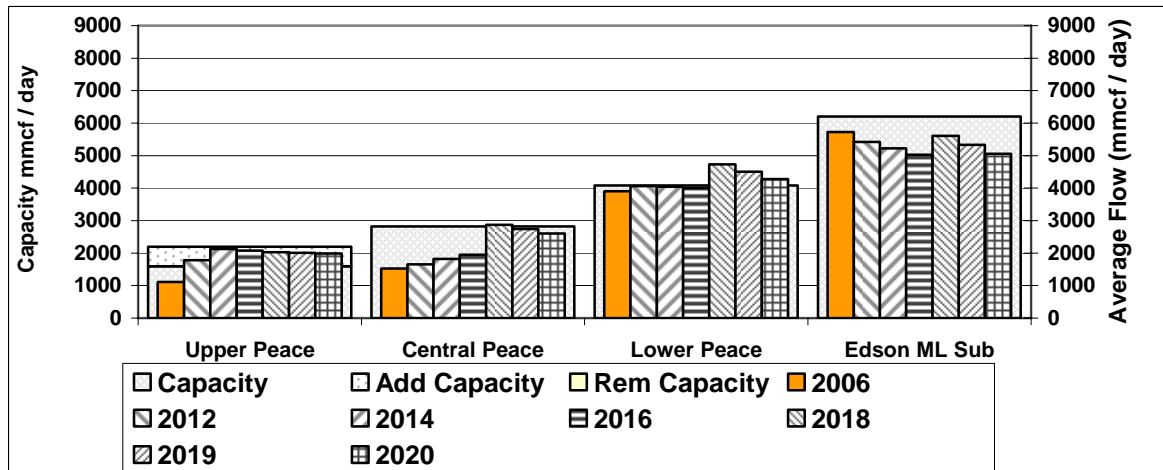
Figure 4.17 Scenario #3 (TCPL/Alliance Transportation) Section Volumes and Capacities (Alberta Northwest)
