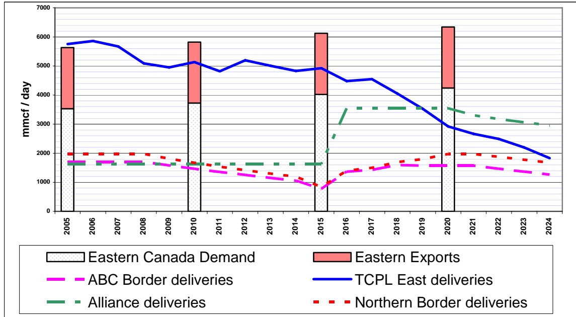
Figure 4.20 Scenario #3 (TCPL/Alliance Transportation)
