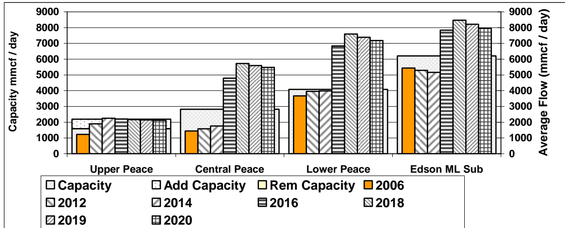
Figure 4.7 Scenario #1 (Utilizing TCPL Integrated System) Section Volumes and Capacities (Alberta Northwest)
