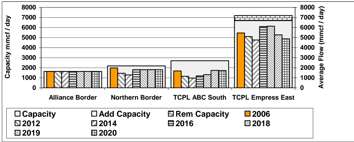
Figure 4.12 Scenario #2 (Utilizing TCPL Integrated System) Section Volumes and Capacities (Alberta Northwest)
