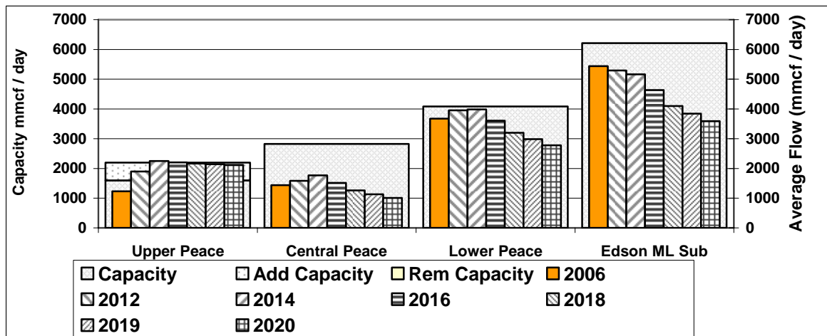
Figure 4.2 Base Case Section Volumes and Capacities (Alberta Northwest)
