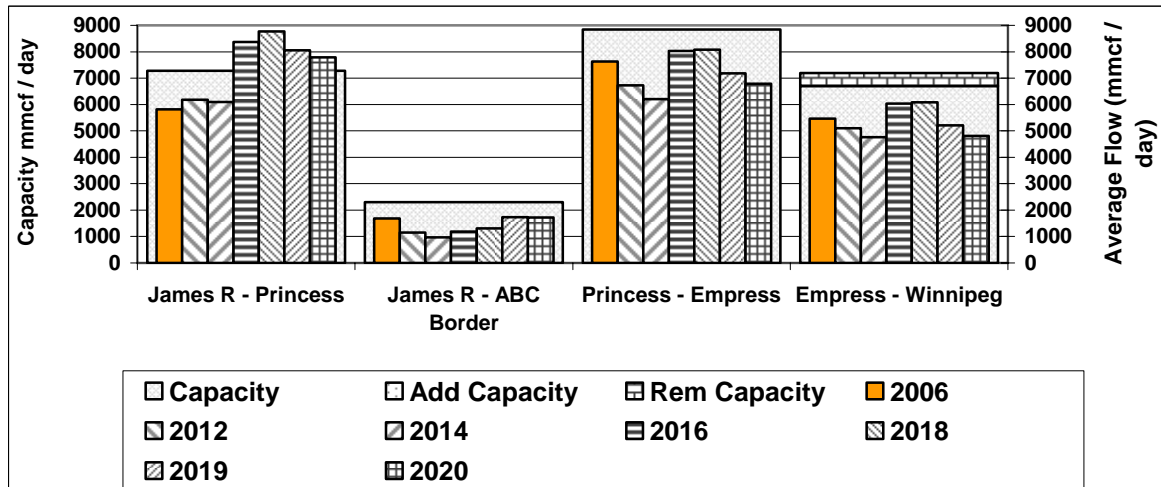
Figure 4.8 Scenario #1 (Utilizing TCPL Integrated System) Section Volumes and Capacities (Alberta Southeast)
