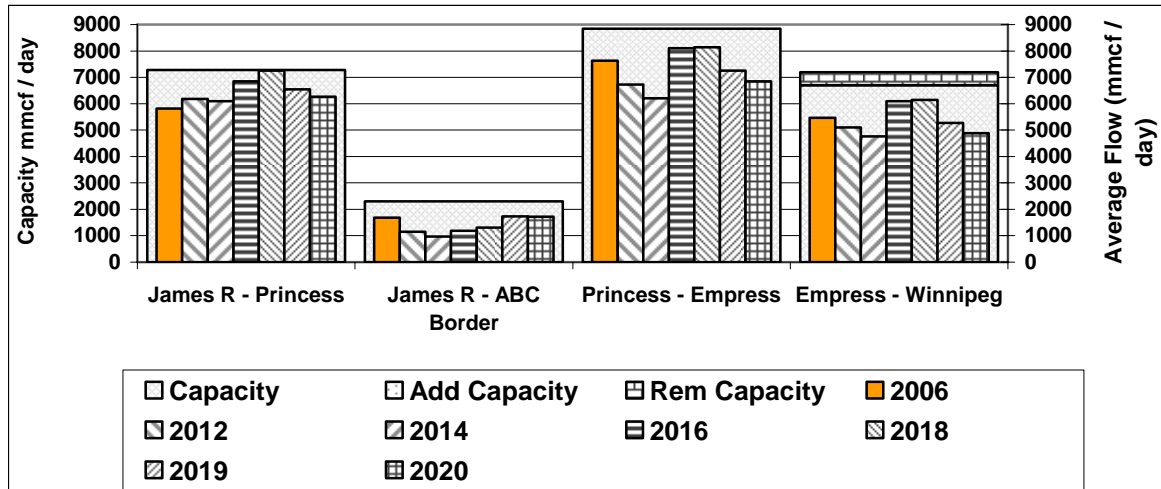
Figure 4.13 Scenario #2 Expanded NCC (Utilizing TCPL Integrated System) Section Volumes and Capacities (Alberta Southeast)
