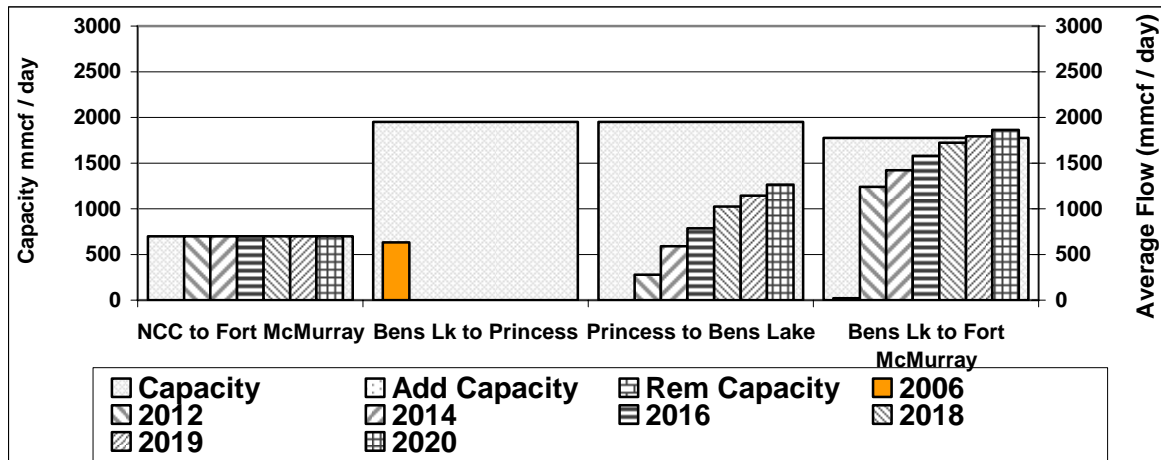
Figure 4.4 Base Case Section Volumes and Capacities (Fort McMurray)
