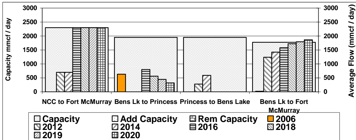
Figure 4.14 Scenario # 2 Expanded NCC (Utilizing TCPL Integrated System) Section Volumes and Capacities (Fort McMurray)
