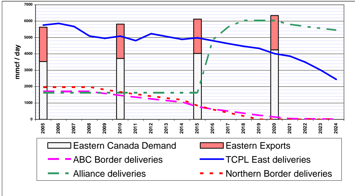
Figure 4.21 Scenario #4 (Alaska Volumes to Alliance 48 inch Capacity)
