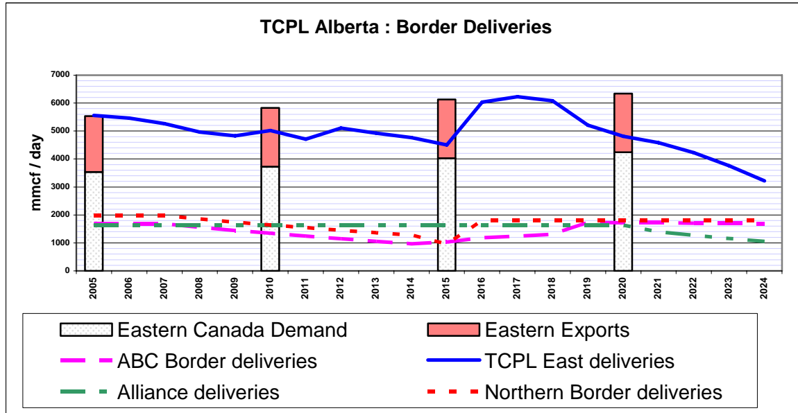
Figure 4.15 TCPL East Canadian Demand and Export Potential
